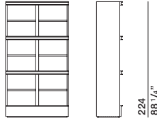
LG/224/121 LGV/224/121 wooden shelves glass shelves
