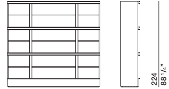
LG/224/241 LGV/224/241 wooden shelves glass shelves
