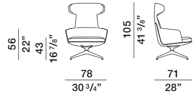
armchair with high back PPA2
