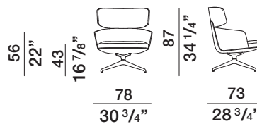
armchair with high back PPA1
