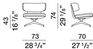
armchair with low back PPB1
