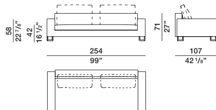
sofa structure DS254
