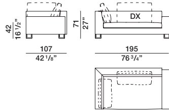
corner element with arm structure ABS195 dx - sx
